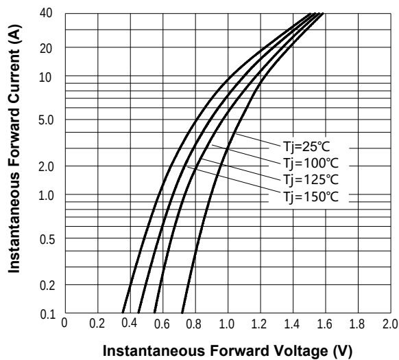
FIG3: Forward Voltage
