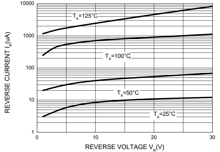
Reverse Characteristics
