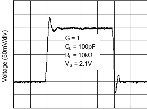
Time (200ns/div)
