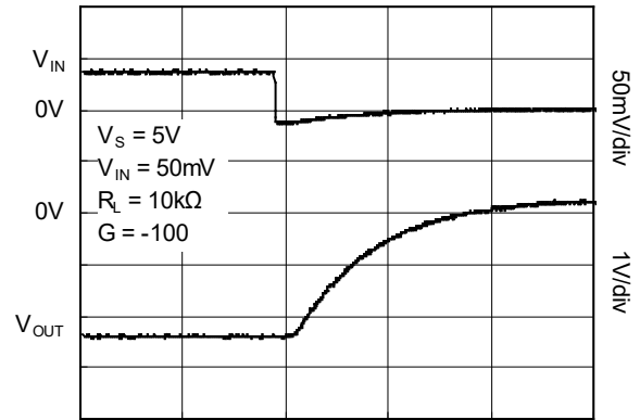
Time (1μs/div)
