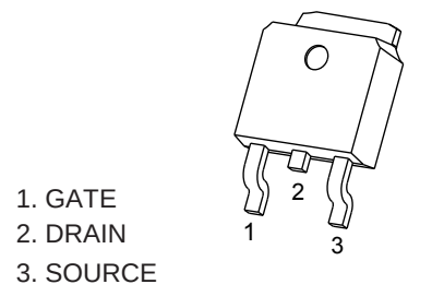
TO-252-2L
