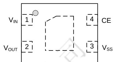
DFN1.2*1.6-4
