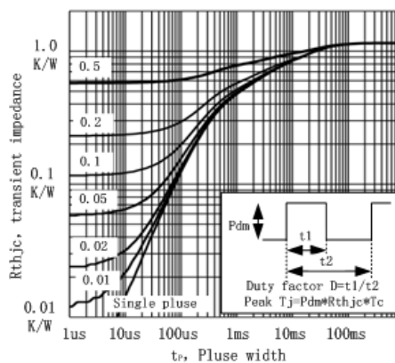
Figure 16 Transient Thermal Impedance of IGBT for TO-220,TO-263
