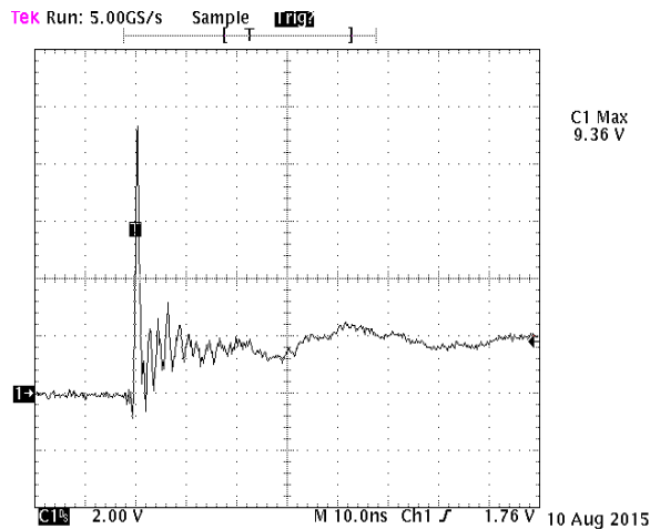
Fig 5. ESD Clamping Voltage Positive 8 kV Contact per IEC61000-4-2
