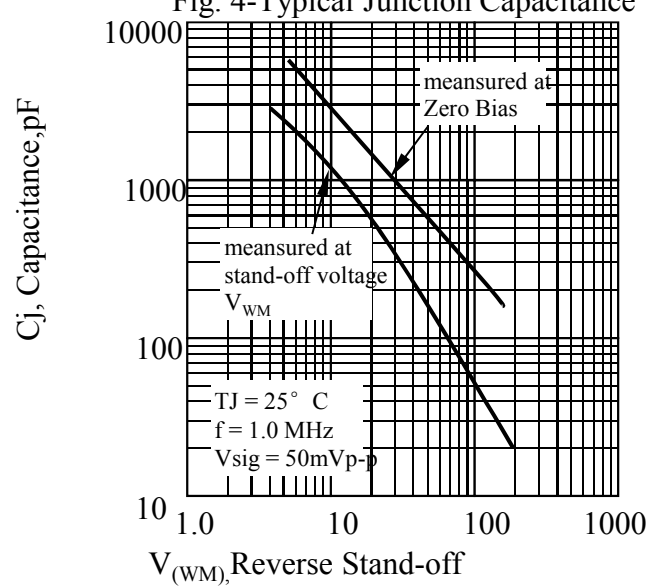
Fig. 4-Typical Junction Capacitance
