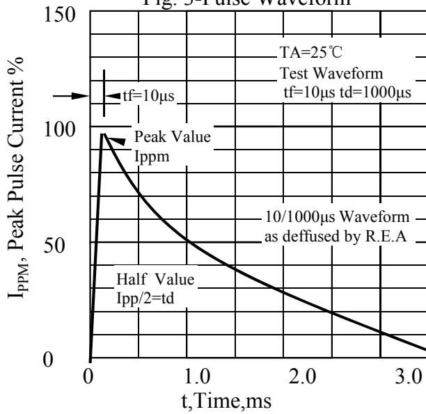
Fig. 3-Pulse Waveform
