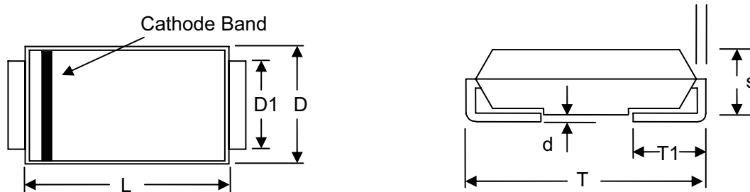
SMC/DO-214AB
