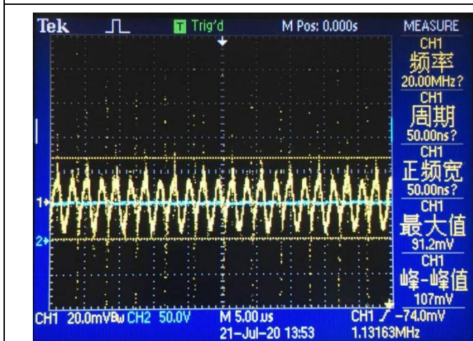
Noise (VIN = 57V, IO = 2A, 5 ~ 20MHz bandwidth)
