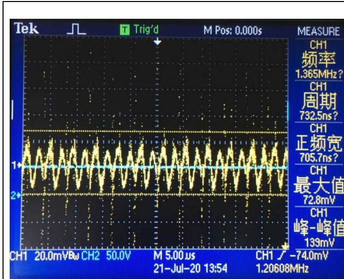
Noise (VIN = 40V, IO = 2A, 5 ~ 20MHz bandwidth)
