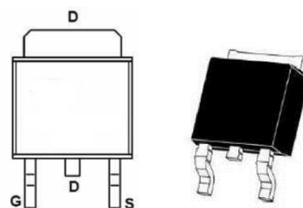
TO-252
