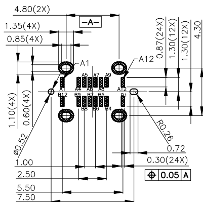
RECOMMENDED PCB LAYOUT(TOP VIEW) THICKNESS 0.8±0.10MM;DEFAULT TOLERANCE:±0.05
