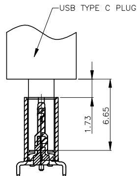
FEMALE AND MALE MATCHING DRAWING
