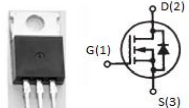
pin 1.Gate 2.Drain 3.Source TO-220 package
