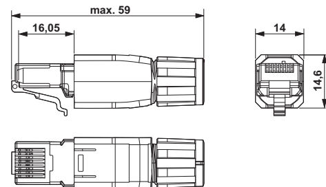
RJ45连接器，IP20
