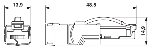
RJ45连接器，IP20
