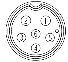
C1 Pin Assignments Front View
