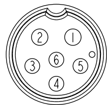
C2 Pin Assignments Front View
