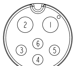
C1 & C2 Pin Assignments Front View
