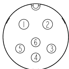
C1 Pin Assignments Front View
