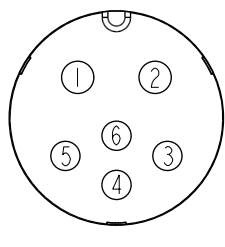
C1 Pin Assignments Front View
