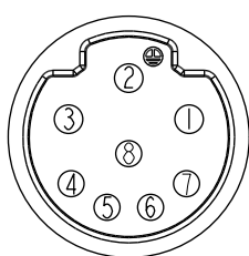
C1 Pin Assignments Front View
