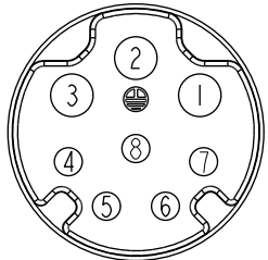
C1 & C2 Pin Assignments Front View
