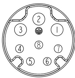
CI Pin Assignments Front View
