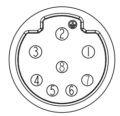
C2 Pin Assignments Front View
