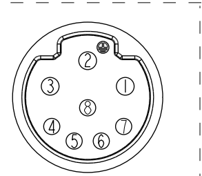
C2 Pin Assignments Front View
