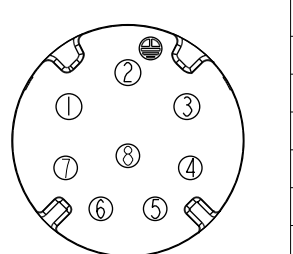
C1 Pin Assignments Front View
