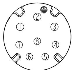
C1 Pin Assignments Front View
