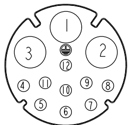
CI Pin Assignments Front View
