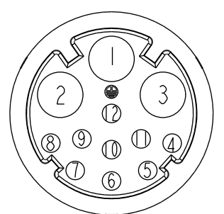
C2 Pin Assignments Front View
