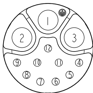
CI Pin Assignments Front View
