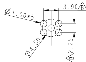
5 Pin Male Connector Male Pin PCB Layout 5 Pin 公座公Pin PCB 挖孔位置尺寸圖
