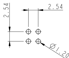
4 Pin Male Connector Male Pin PCB Layout
