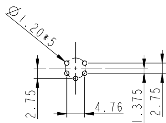
5 Pin Male Connector Female Pin PCB Layout
