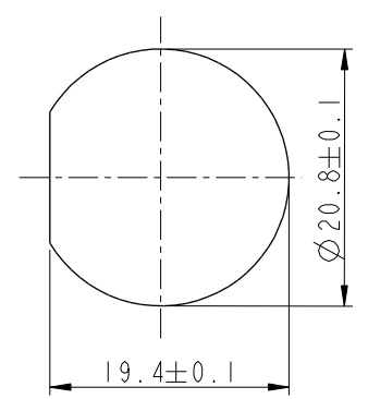
Recommenderd Panel Cut-Out
