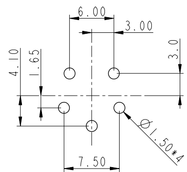
5Pin Male Connector Male Pin PCB Layout
