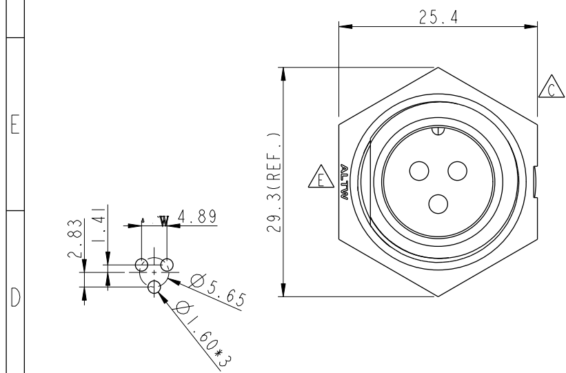
3Pin Male Connector Female Pin PCB Layout
