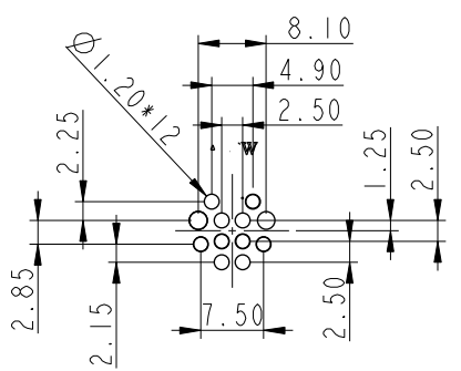
12Pin Male Connector Female Pin PCB Layout
