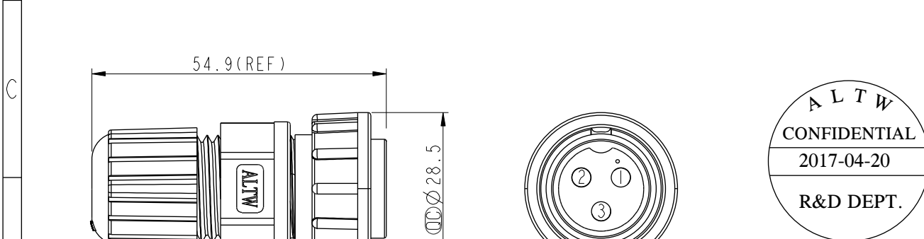
Pin Assignments Front View
