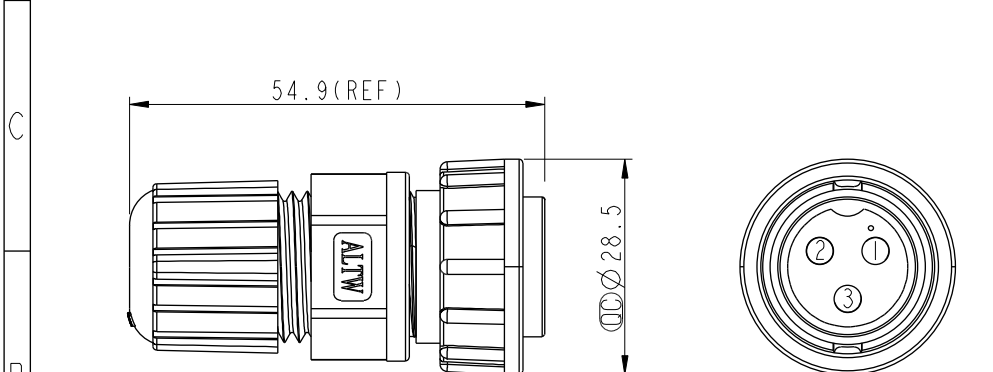
Pin Assignments Front View
