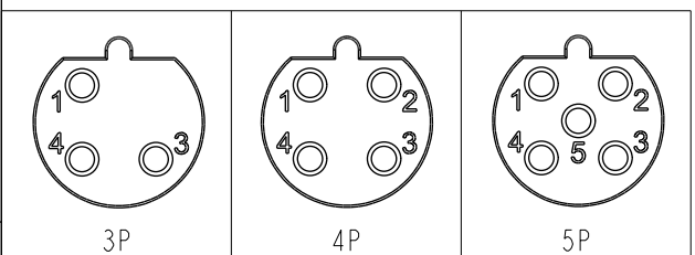
Pin Assignments Front View
