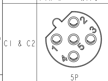
Pin Assignments Front View
