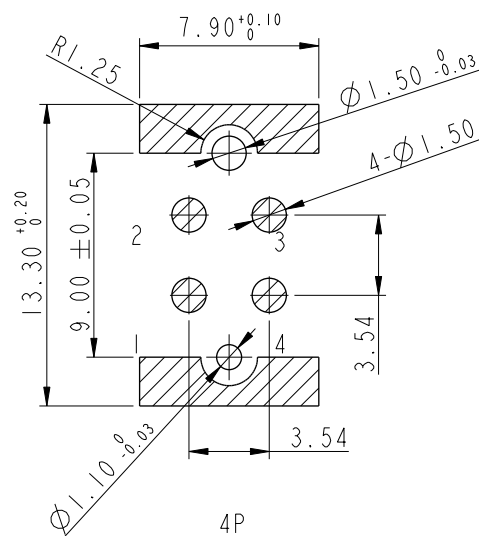
PCB Layout
