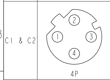
Pin Assignments Front View
