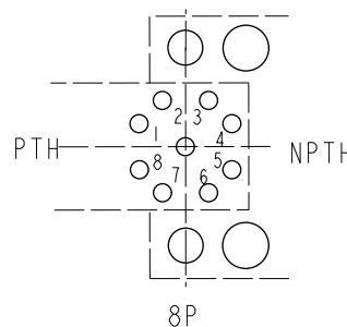
Pin Definition
