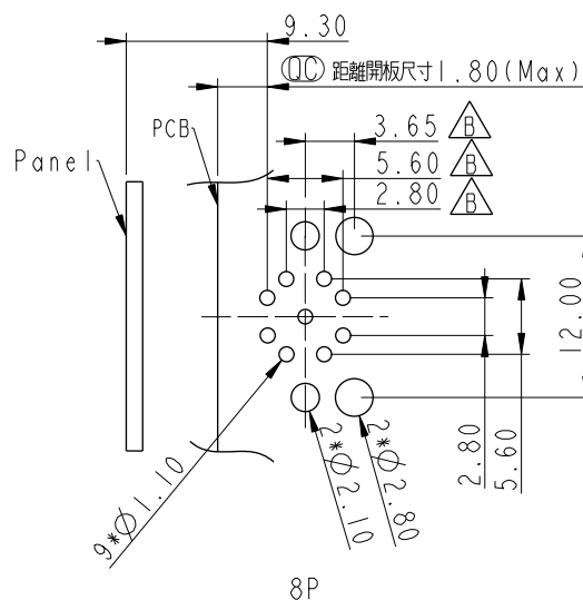
PCB Layout
