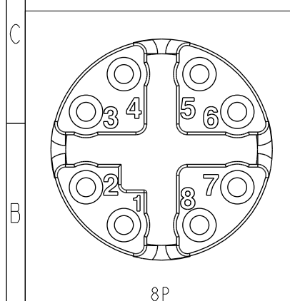
△ Pin Assignment Front View
