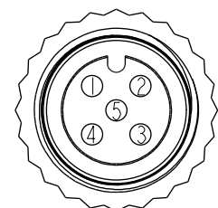
Conn. I Pin Assignments Front View
