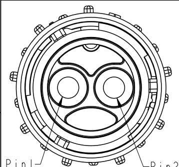
Pin1 Pin2 Pin Assignments Front View
